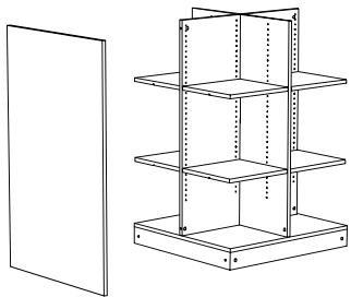
End Panels can be added to or removed from Bins without removing Shelves.
